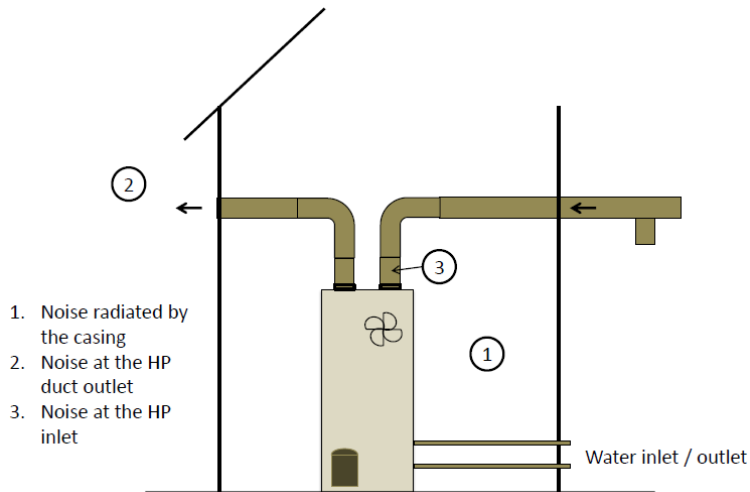
Figure 1: Acoustic measurements on air exhaust air-to-water heat pumps
